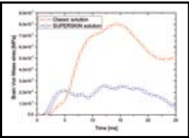
Intracerebral stress Von Mises yield criterion
