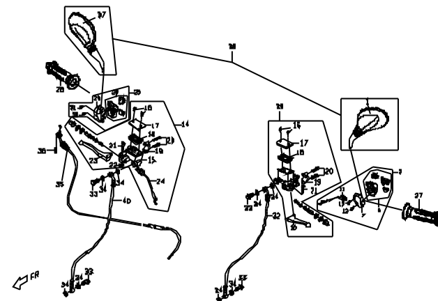
F3.2 導線開關。後視鏡 (前碟後碟) CABLE SWITCH BACK MIRROR
