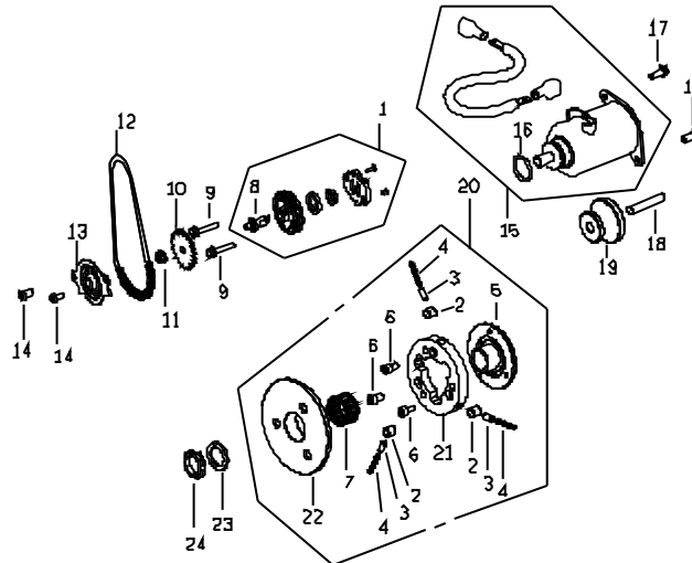
E9 起動馬達 STARTING MOTOR, OIL PUMP
