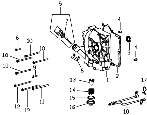
E5 右曲軸箱蓋 RIGHT CRANKCASE COVER
