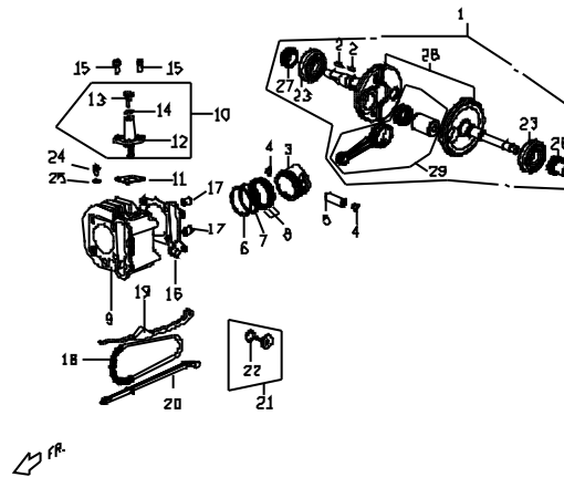
E4.1 曲軸及汽缸 (125 CC) CYLINDER . PISTON . CRANKSHAFT
