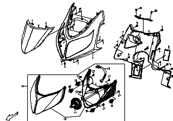
F6 擋風板。前內蓋。前大燈 WINDSHIELD.FRT INNER COVER. FRT HEAD LIGHT.
