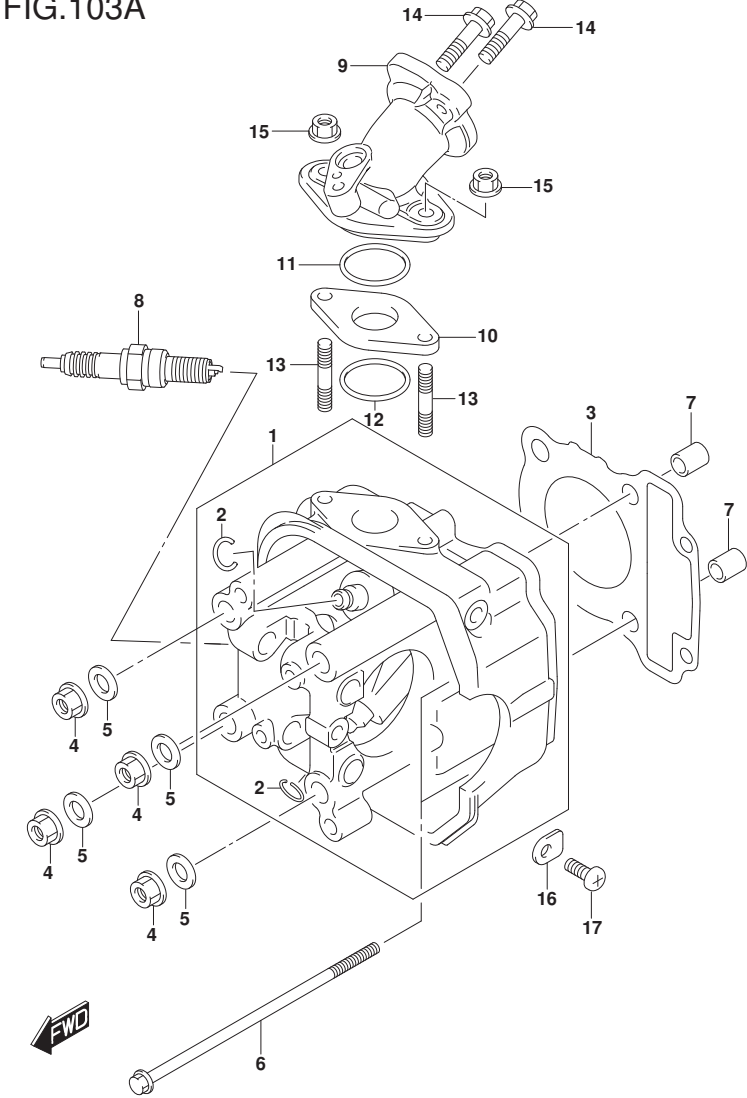
UG125L9_N00_103A CYLINDER HEAD
