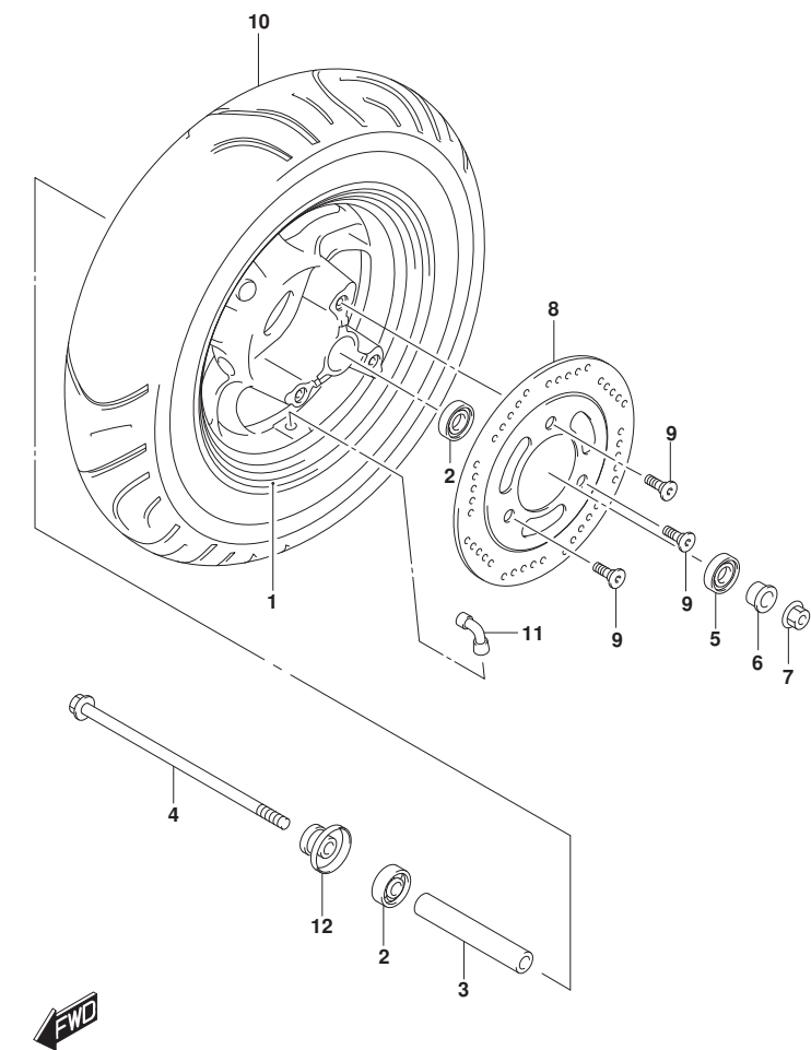
UG125L9_N00_530A FRONT WHEEL
