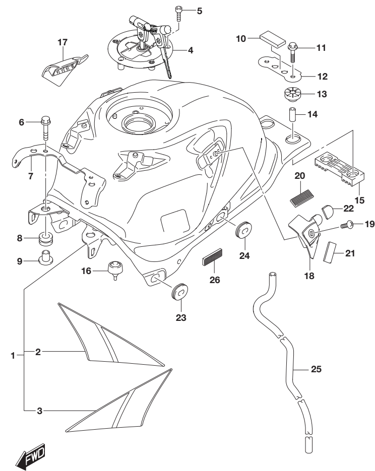
GSX-S125XAM0_N00_420A FUEL TANK
