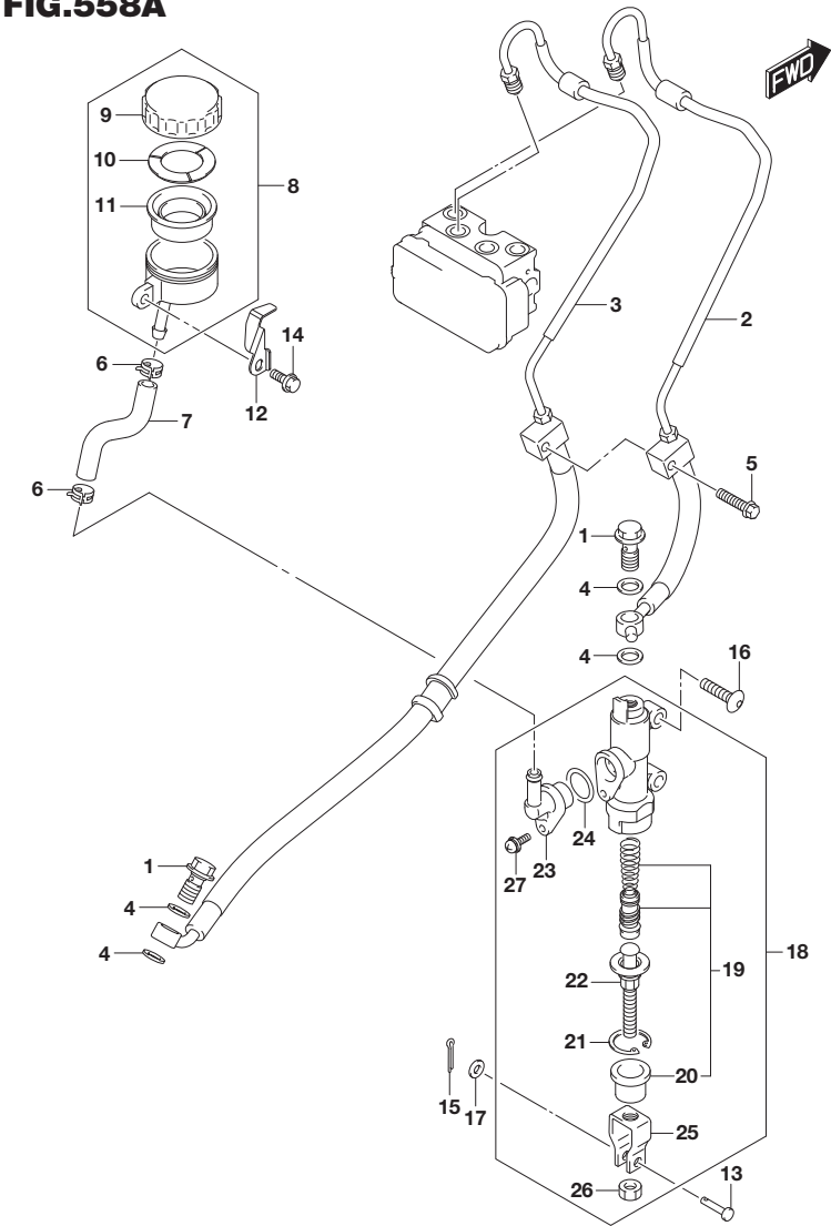
GSX-R125M0_N00_558A REAR MASTER CYLINDER
