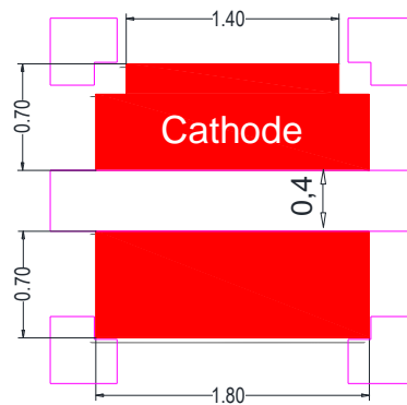
< Recommended Solder Pattern >
