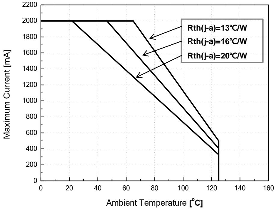
Fig 9. Maximum Forward Current vs. Ambient Temperature, T_j(\text{max.})=145^\circ\text{C} , I_F=2.0\text{A}
