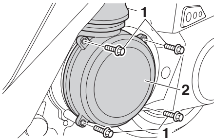
1. 螺栓 (x4)
