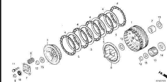
E-8 CLUTCH
