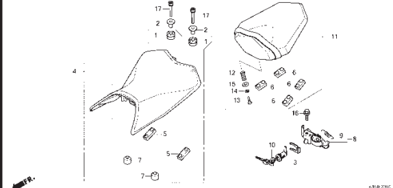
F-23 SEAT
