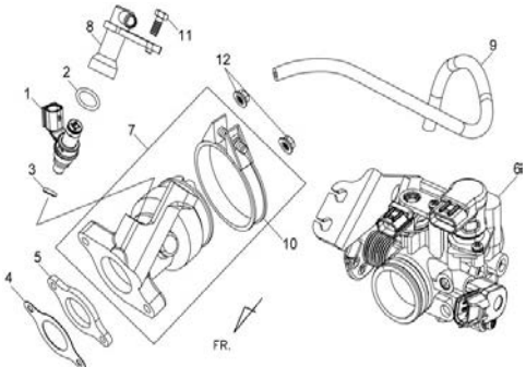
E19 IN PIPE&THROTTLE BODY ASSY
