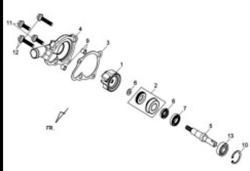
E21 WATER PUMP COVER ASSY
